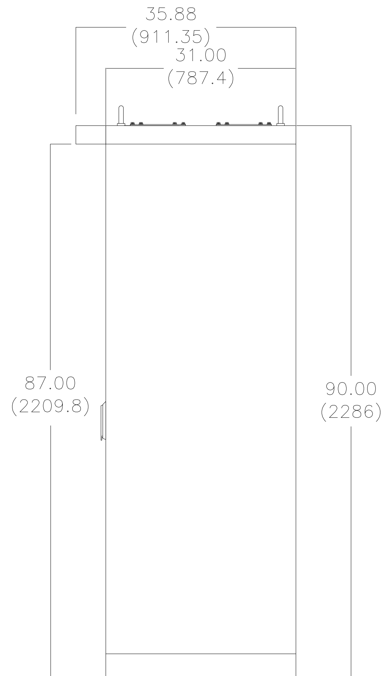
SIDE VIEW
