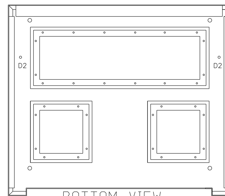
BOTTOM VIEW SECTION B-B
