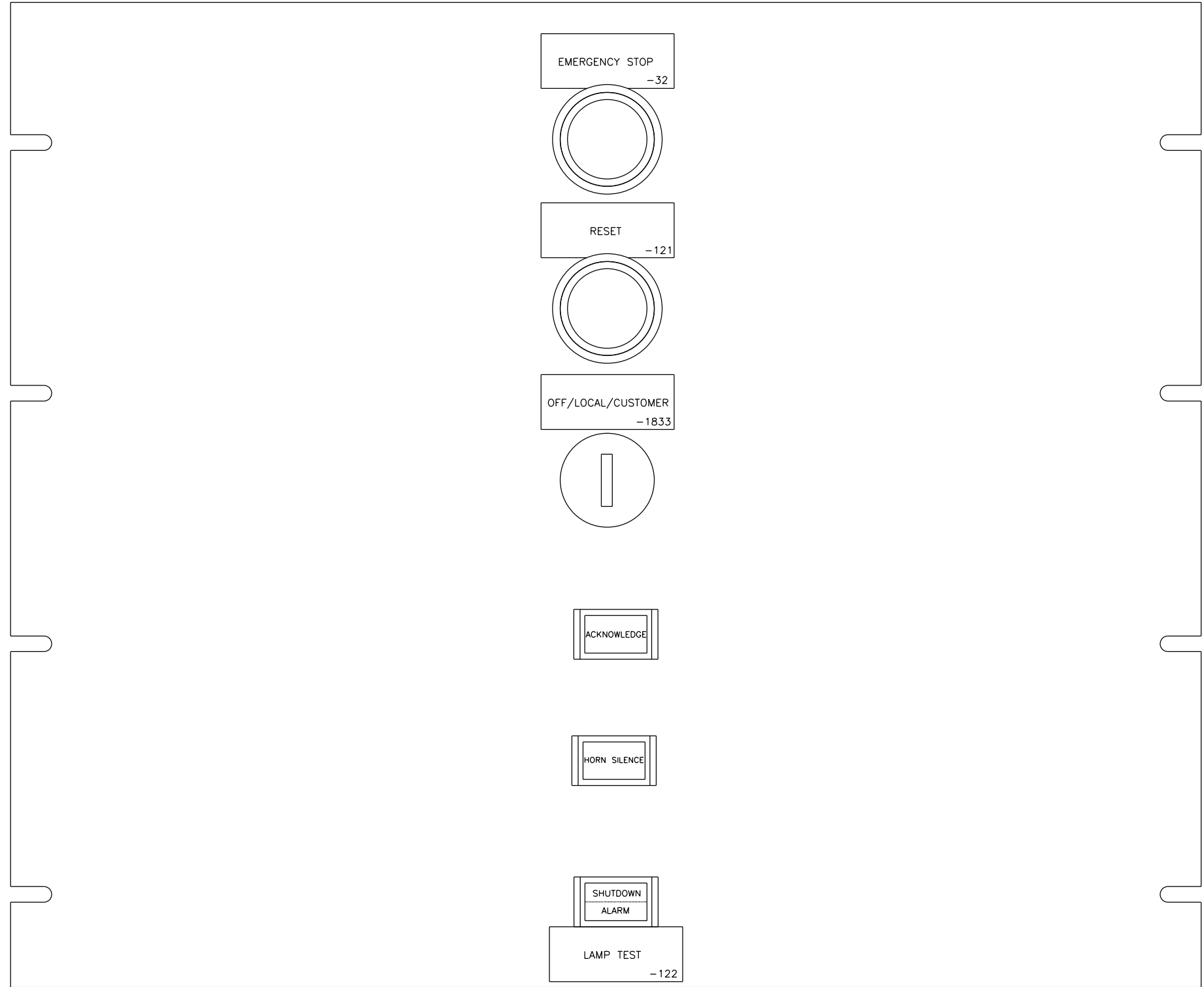
FRONT VIEW
