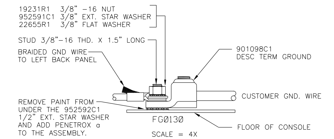
TYPICAL GROUND STUD ASSEMBLY
