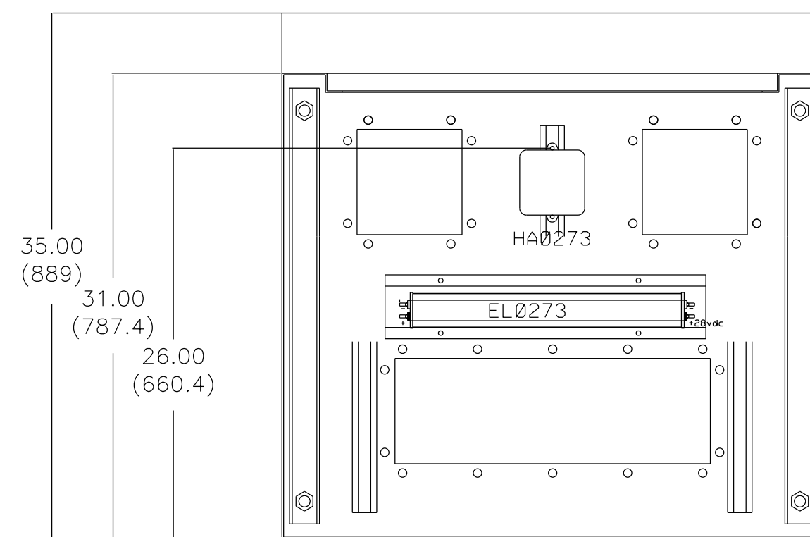
TOP VIEW SECTION A—A
